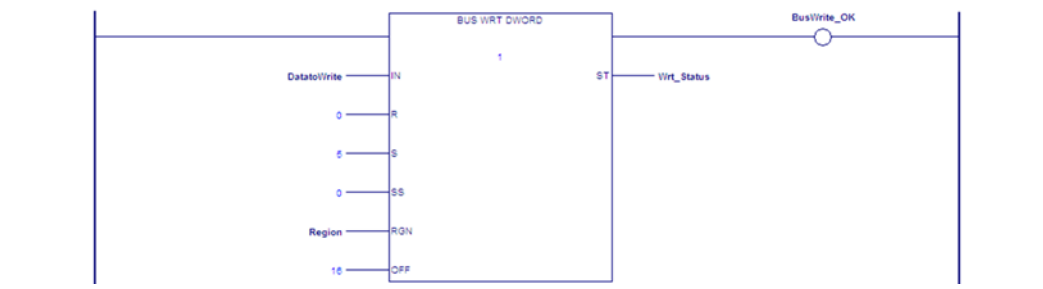
Figure 9: Sample Ladder Logic for BUS_WRT_DWORD function
