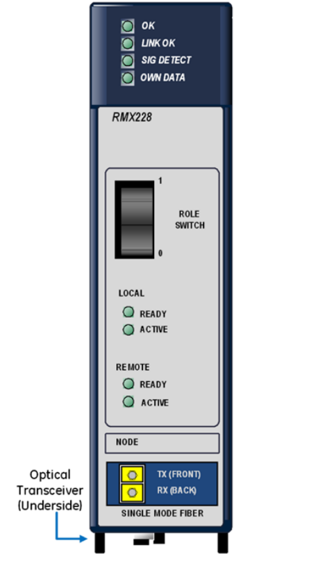
Figure 13: RMX228 Features
