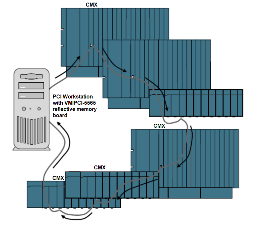
Figure 1: 7-Node Reflective Memory Network
