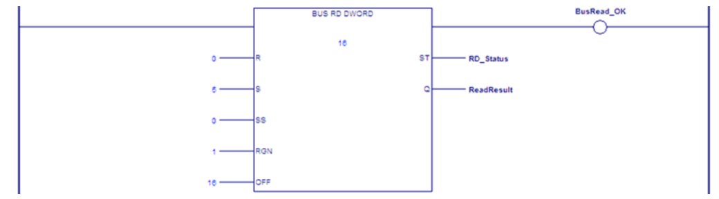
Figure 10: Sample Ladder Logic for BUS_RD_DWORD function
