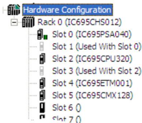
Figure 6: PAC Machine Edition Hardware Configuration
