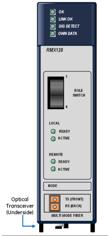
Figure 12: RMX128 Features
